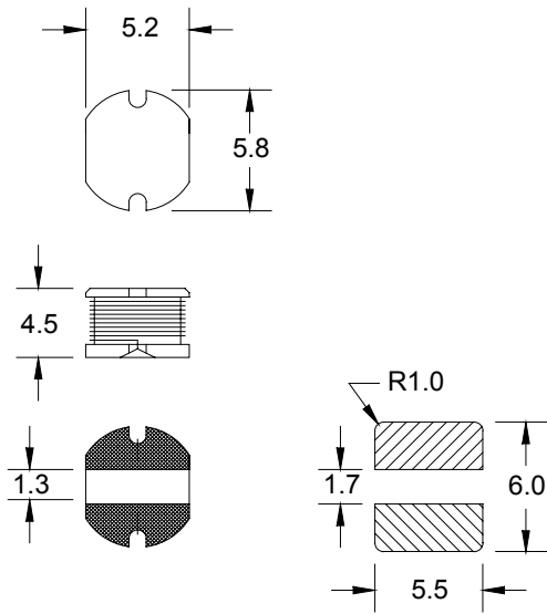
Pad Layout
